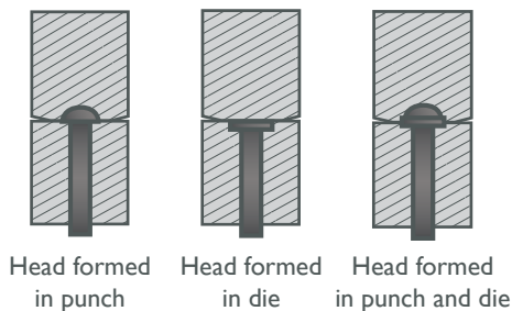
Cold-heading rams material into the void of a die or punch forcing the metal to reshape itself to fill the void.
