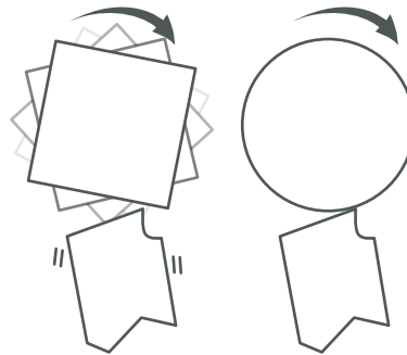
INTERRUPTED VS. SMOOTH CUT
